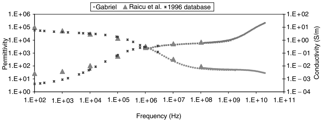
FIGURE 3.22 Permittivity and conductivity of skin (Raicu et al.: back of neck, moistened with physiological saline; Gabriel and database: ventral forearm, moistened with water). Open-ended coaxial probes of vastly different sizes were used.
