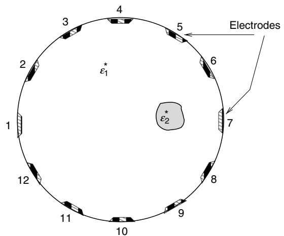
FIGURE 12.5 Configuration of electrical impedance tomography.
