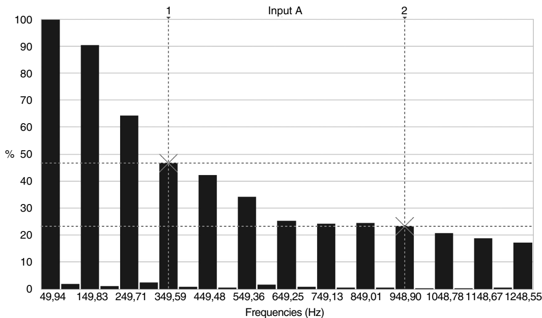
FIGURE 1.11 The Fourier spectrum of the wave shape in Figure 1.7. Note the high 150-Hz component. (Figure courtesy of Swedish National Institute for Working Life.)
