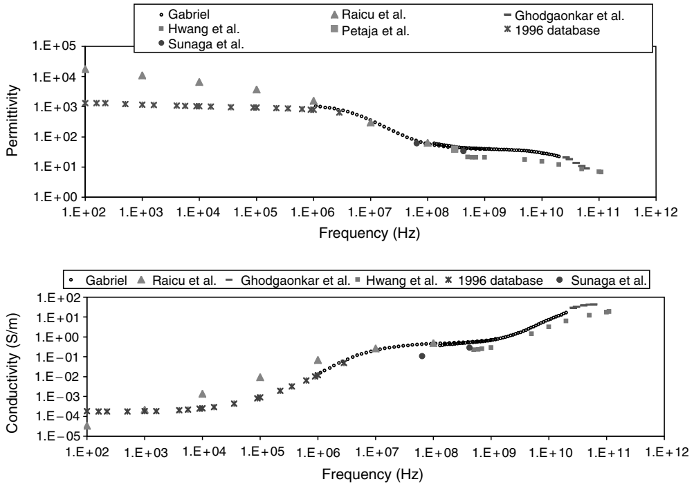
FIGURE 3.21 Permittivity and conductivity of skin (different parts of the body, excluding palms and soles). No moistening or contact gel was used. Different measurement techniques were used including open-ended coaxial probes of vastly different sizes.
